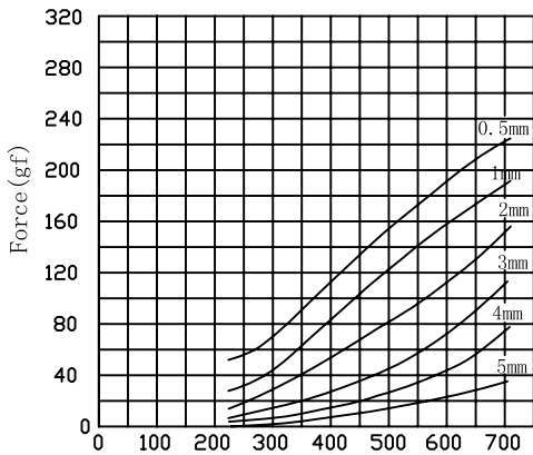
Ampere-turns (AT)
